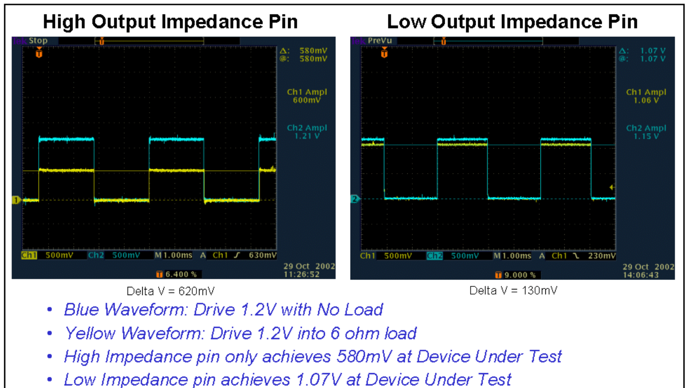
Figure 3: Driver Accuracy Comparison
