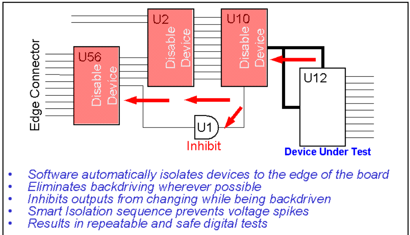
Figure 9: Multi-Level Digital Isolation
