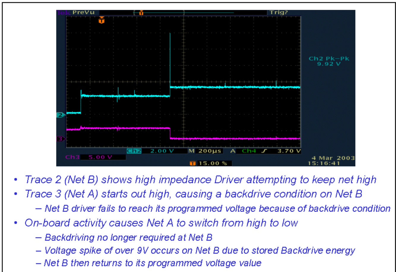
Figure 7: Voltage Spike Resulting from Output Changing During Backdrive
