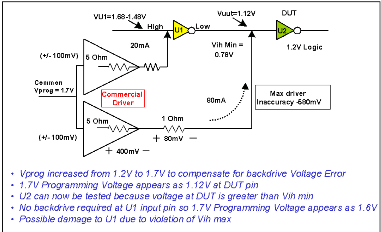
Figure 4: Shared Logic Level Assignments Causing Over-voltage Condition
