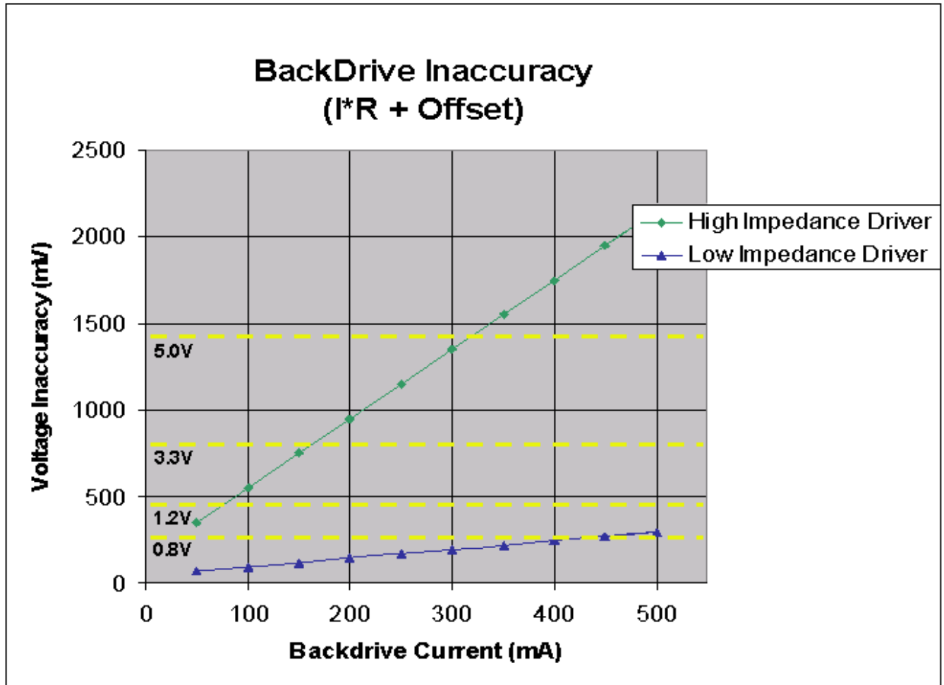
Figure 2: Driver Inaccuracy Increases as Backdrive Current Increases
