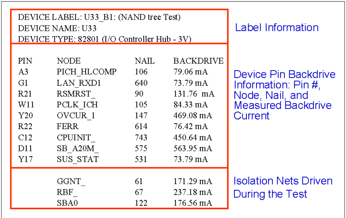
Figure 5: ICT Report Showing Backdrive Currents
